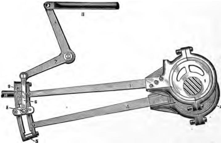
FIG. 329.—Diagram of the Link Motion and Eccentric Gear of a Steam Engine. The parts shown are: (1) backward eccentric; (2) forward eccentric; (3-4) eccentric rods; (5) slotted shifting link; (6) link hanger; (7) reversing arm; (8) link saddle pin; (9) link block; (10) valve stem; (11) reach rod. The position shown in the cut indicates that the backward eccentric is in gear which gives a reverse motion to the engine.
